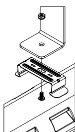
Trunnion Mount
