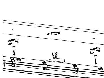
Junction Mount
